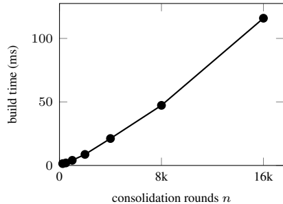
(a) integer codes: build vs n
