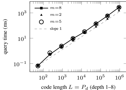
(b) padded codes: query vs. |\text{code}|
