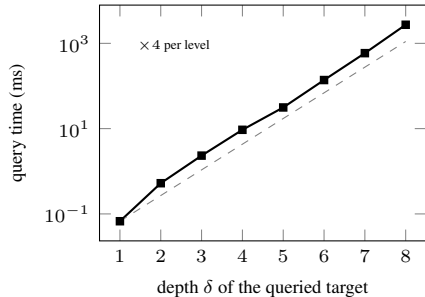
(c) padded codes: query vs. depth ( m=8 )
