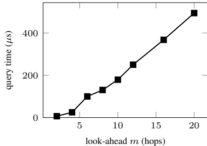
(b) query vs. look-ahead, n = 8000
