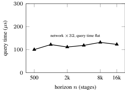
(c) horizon-uniformity, m = 8
