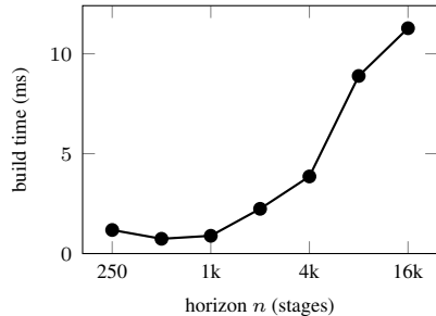
(a) materialization: linear in n
