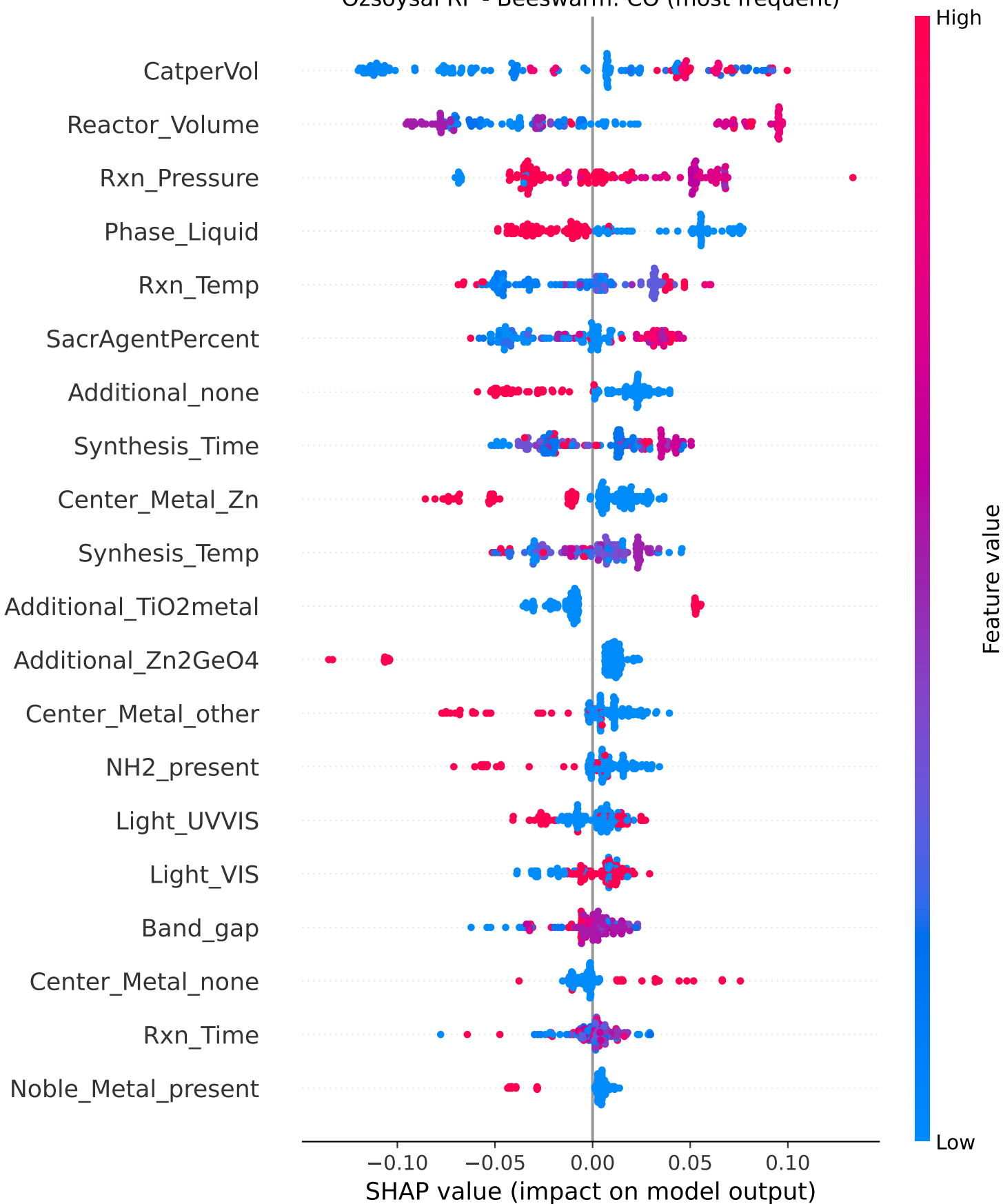
Ozsoysal RF - Beeswarm: CO (most frequent)
