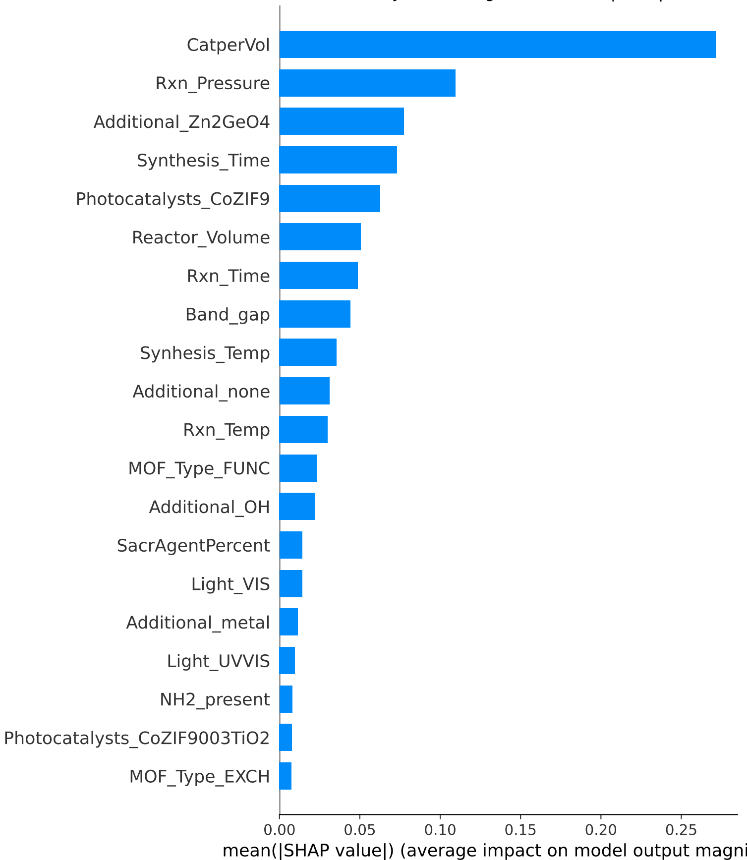
Ozsoysal RF - Regression: Mean |SHAP|
