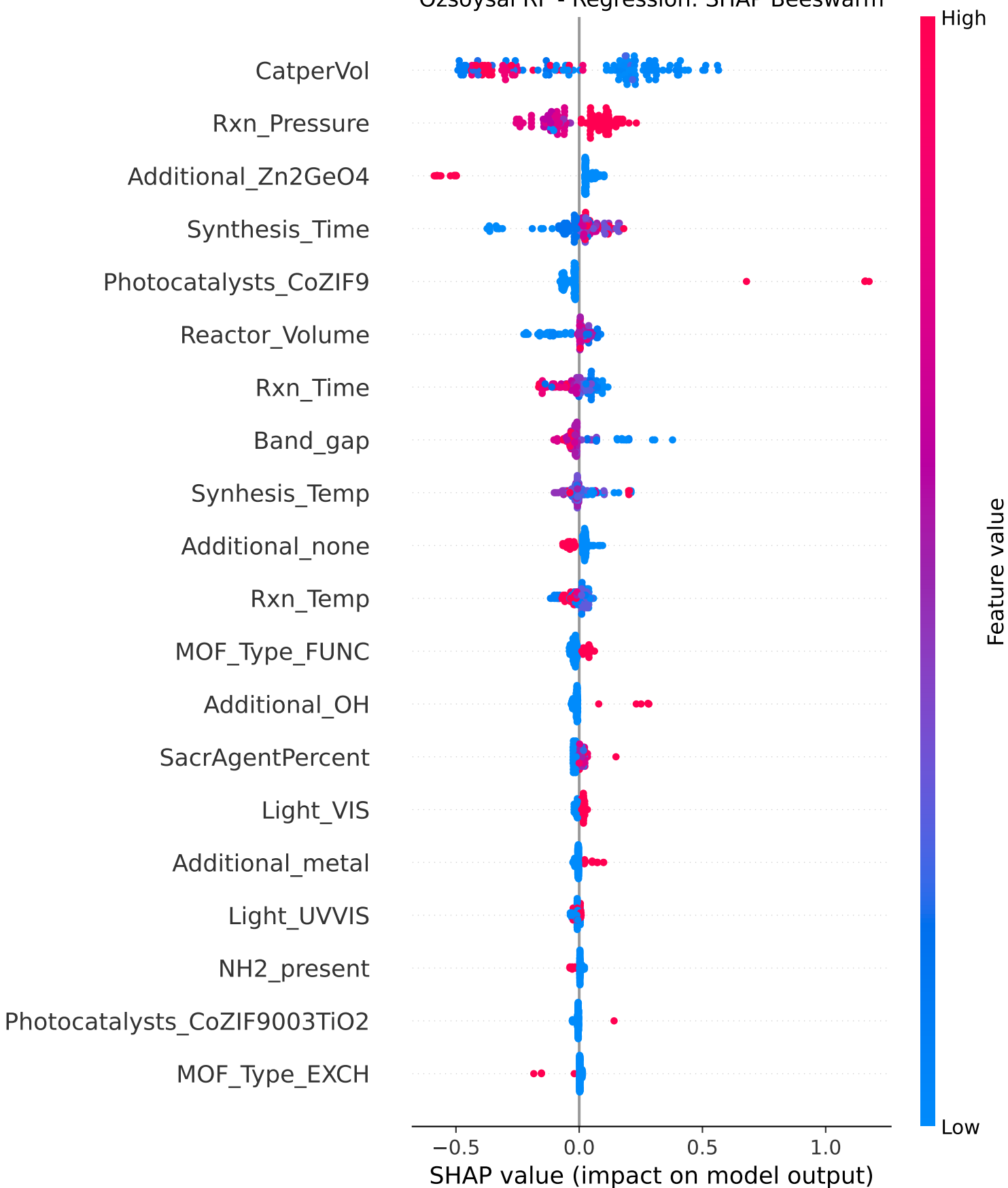
Ozsoysal RF - Regression: SHAP Beeswarm
