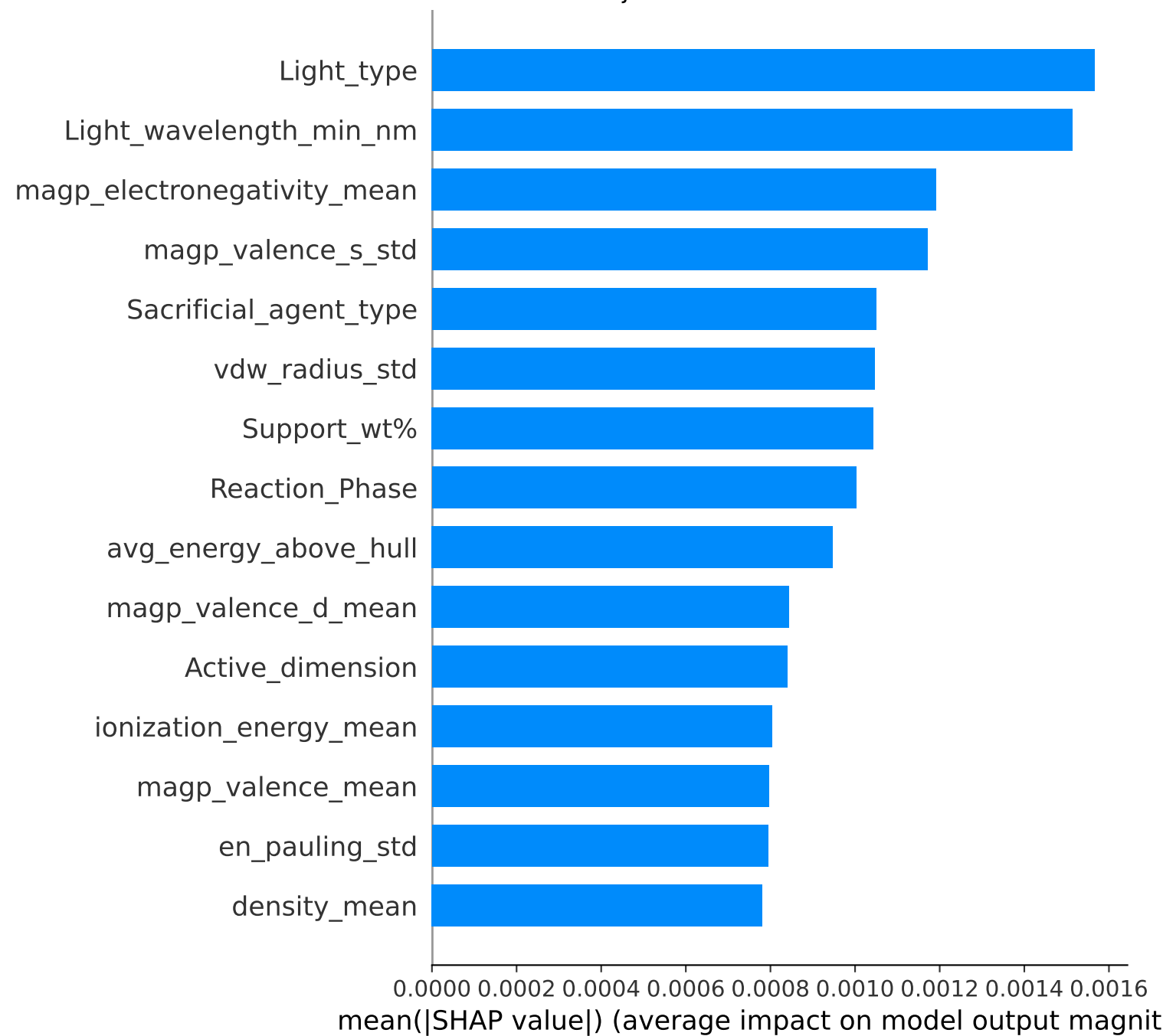
Major Product -- Class: C2H5OH
