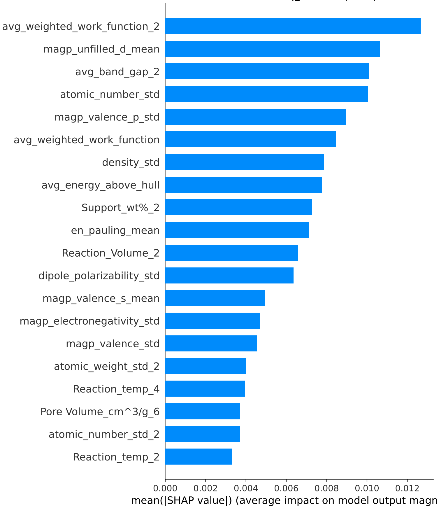
PRIDMO RF - Mj_clf: Mean |SHAP|
