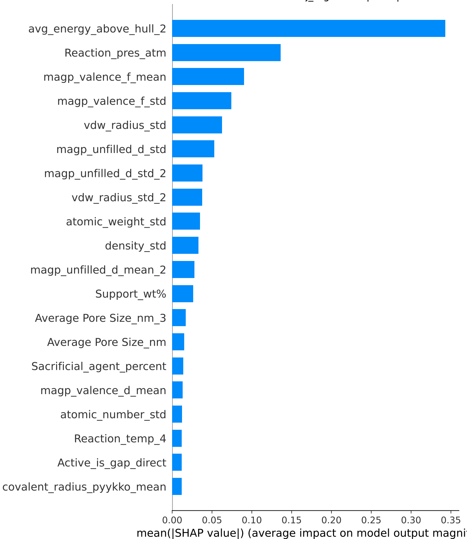
PRIDMO RF - Mj_reg: Mean |SHAP|
