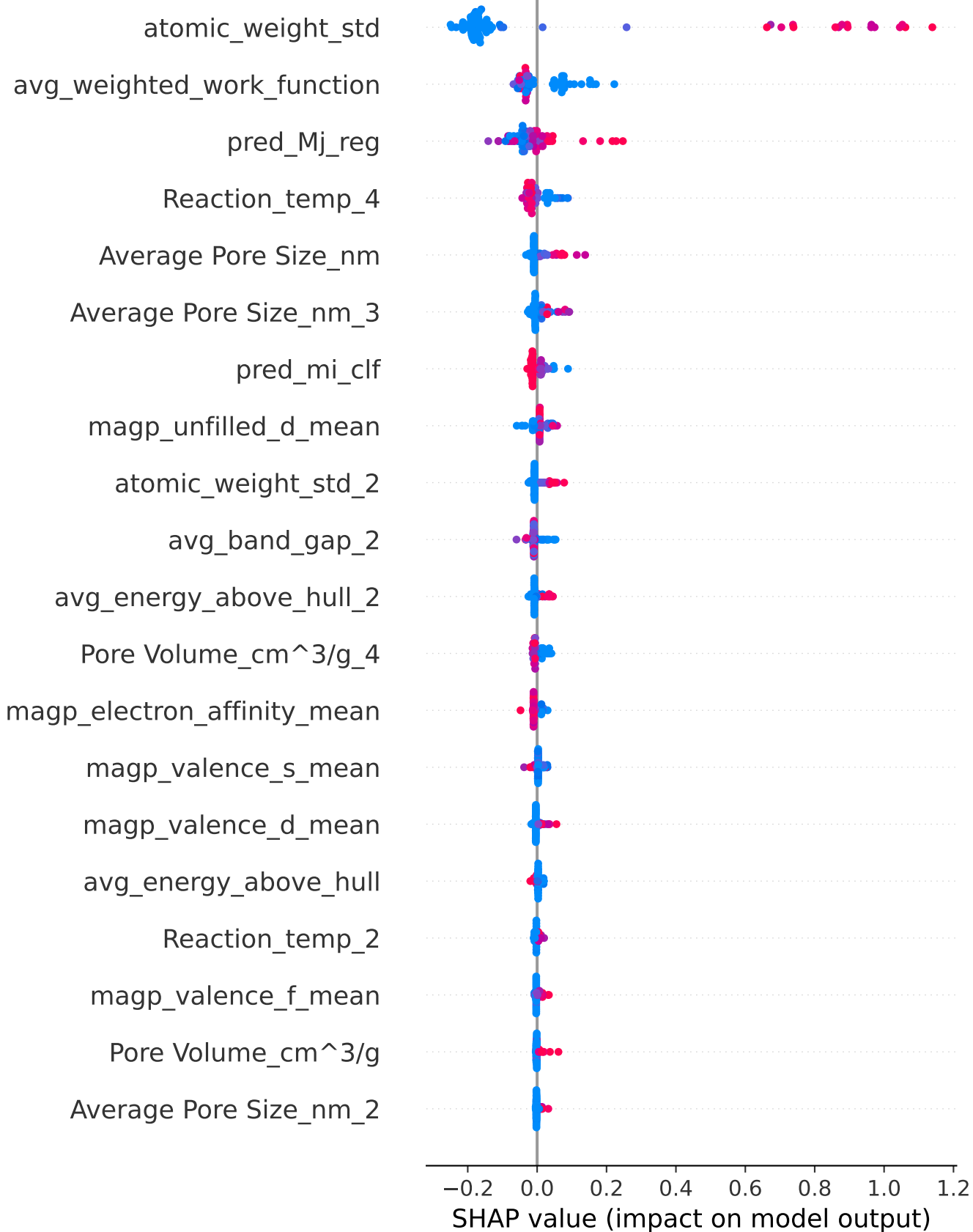
PRIDMO RF - mi_reg: SHAP Beeswarm
