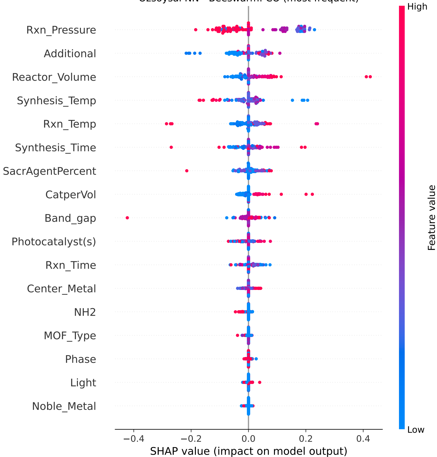
Ozsoysal NN - Beeswarm: CO (most frequent)
