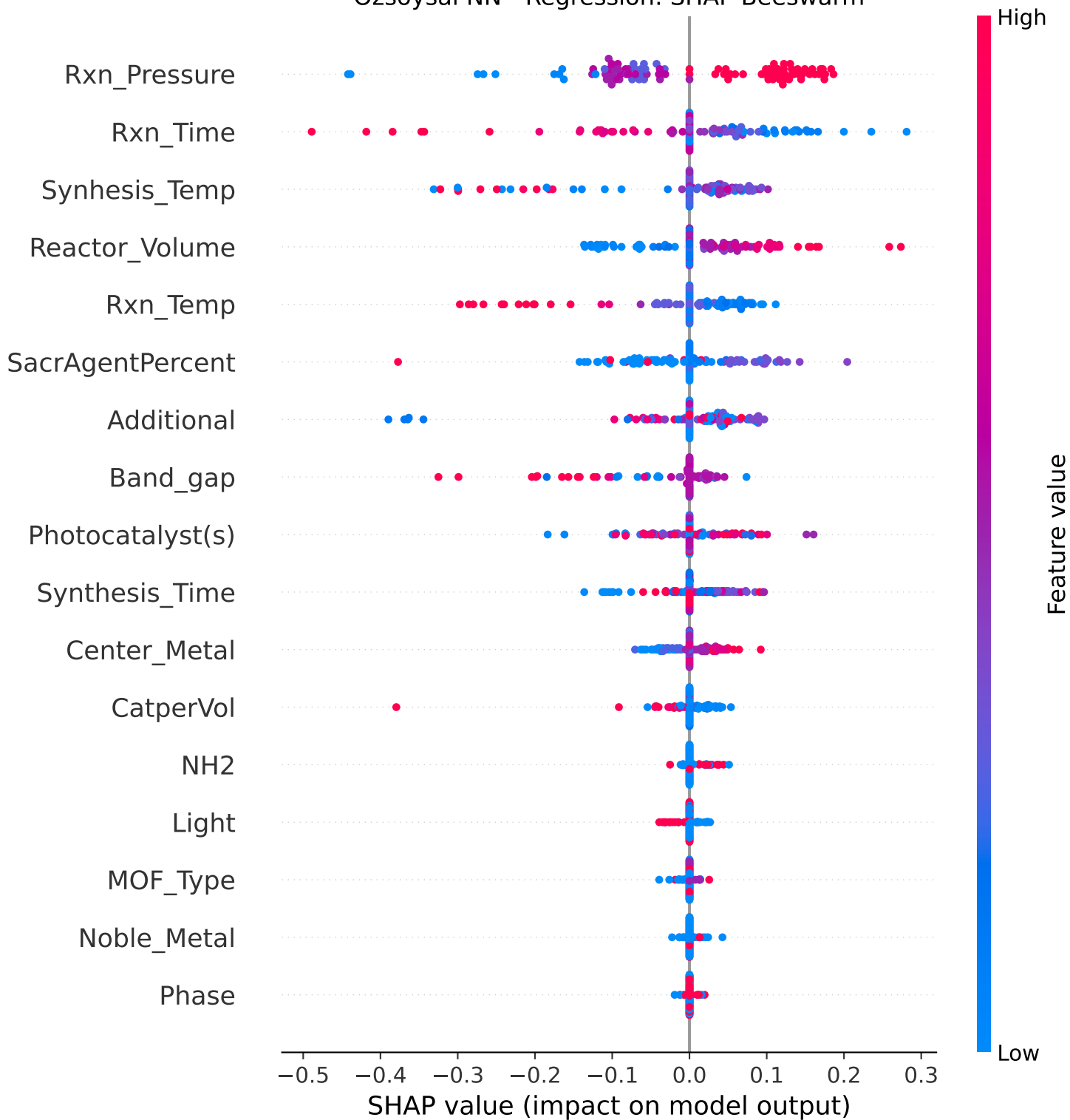
Ozsoysal NN - Regression: SHAP Beeswarm
