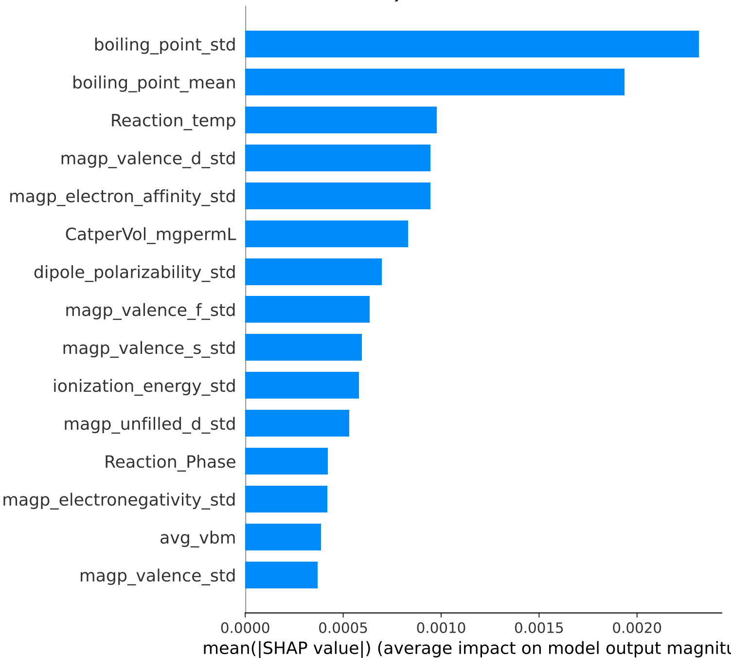
Major Product -- Class: C3H6
