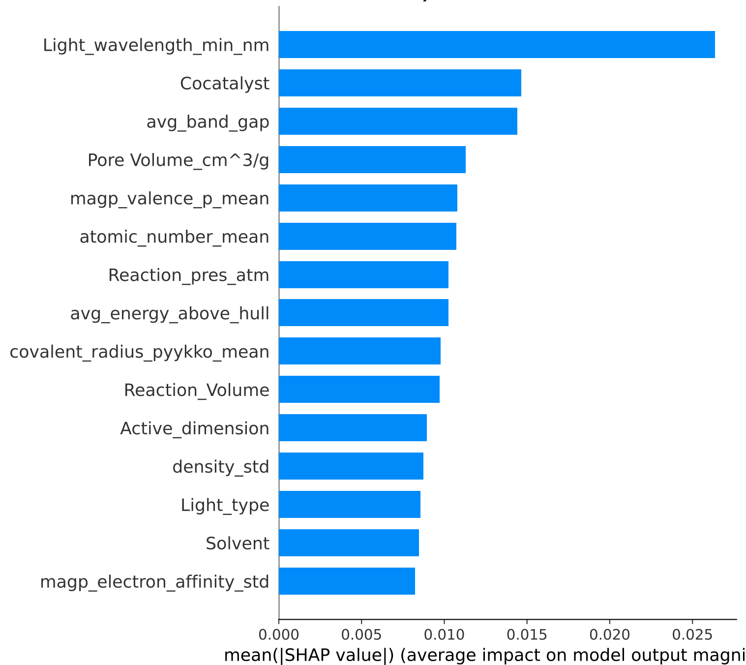
Major Product -- Class: CH4
