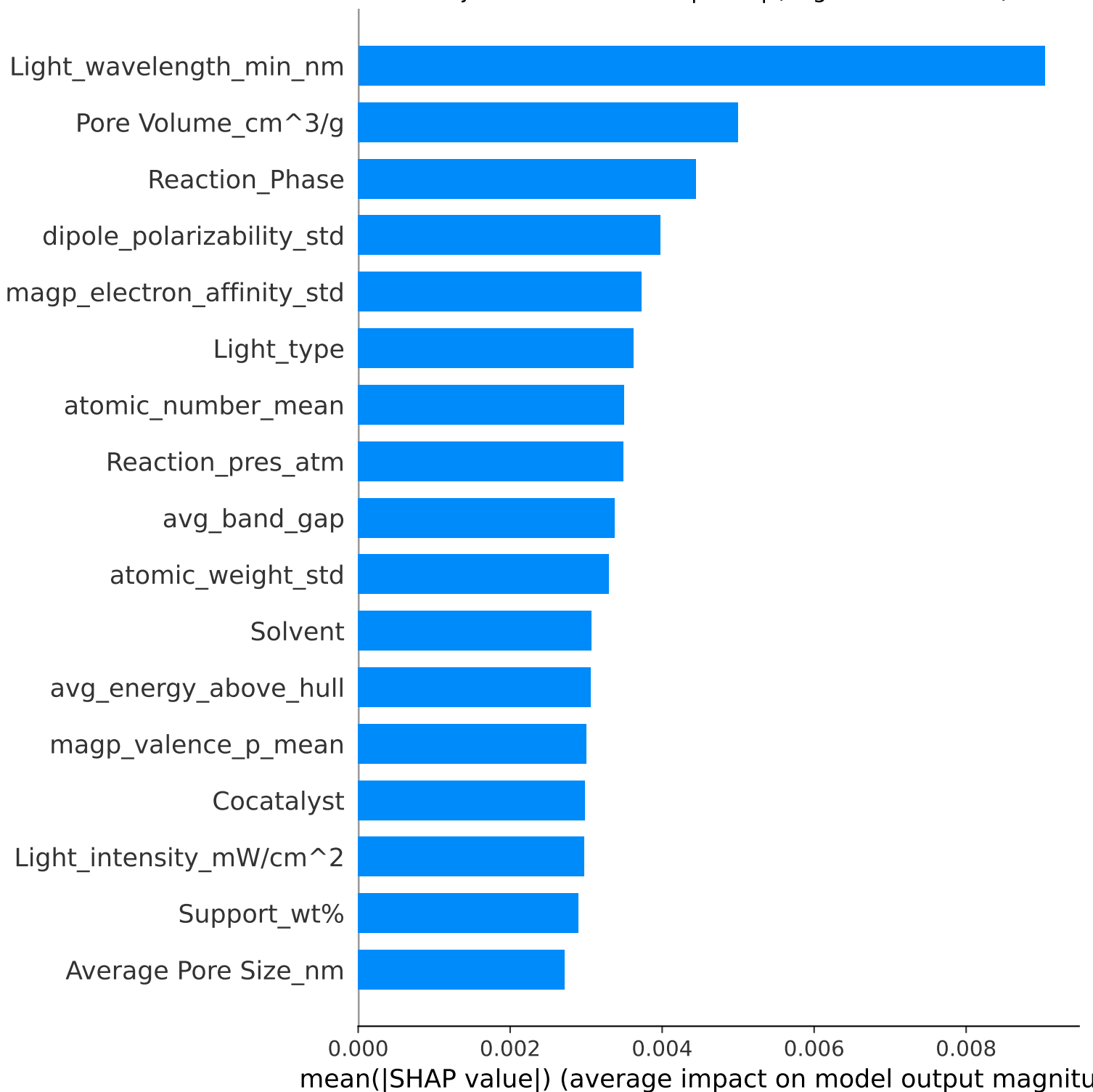
Major Product -- Mean |SHAP| (avg across classes)
