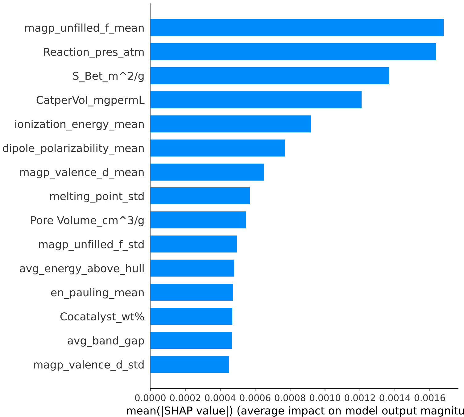
Minor Product -- Class: C2H4
