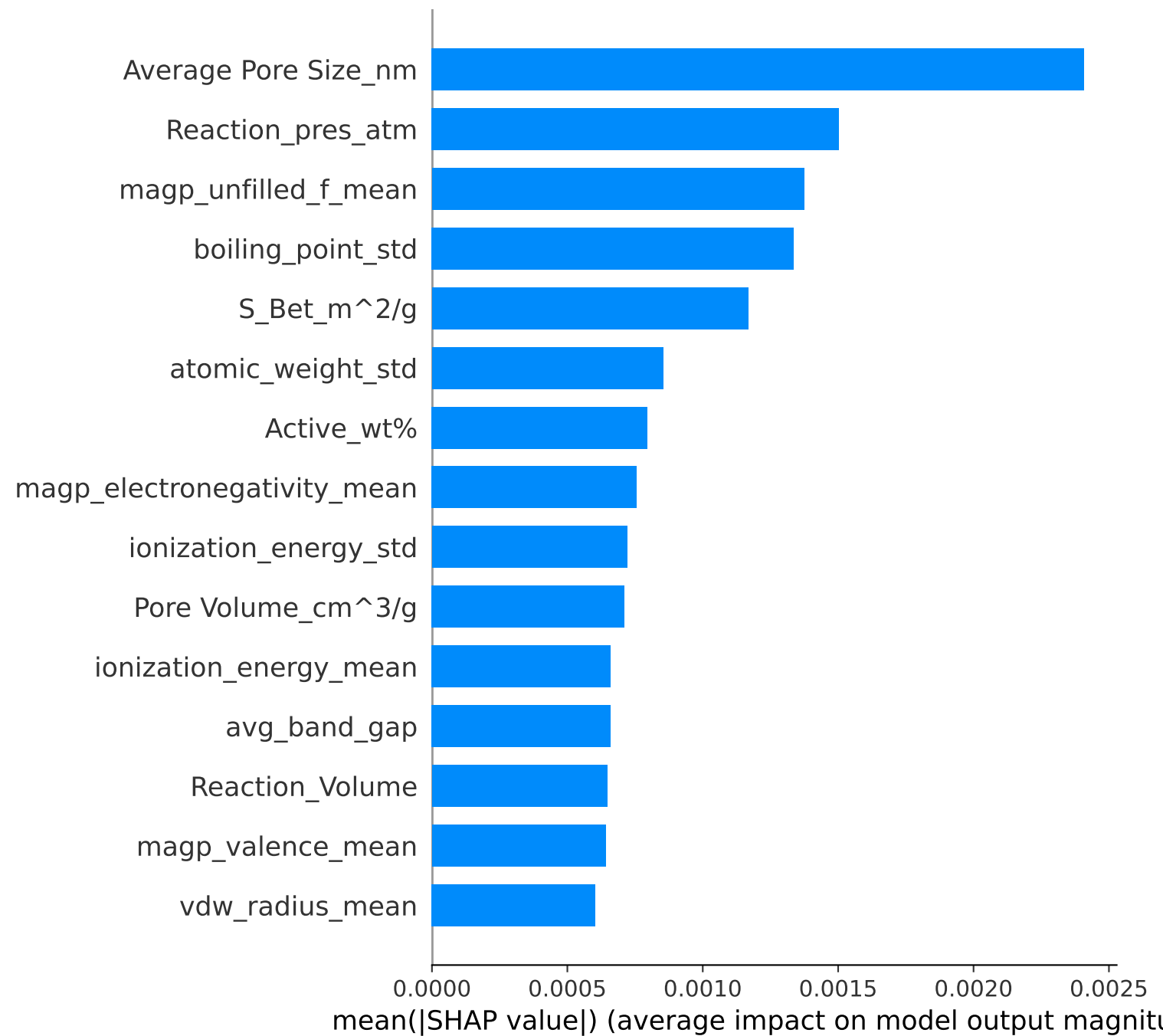
Minor Product -- Class: HCHO
