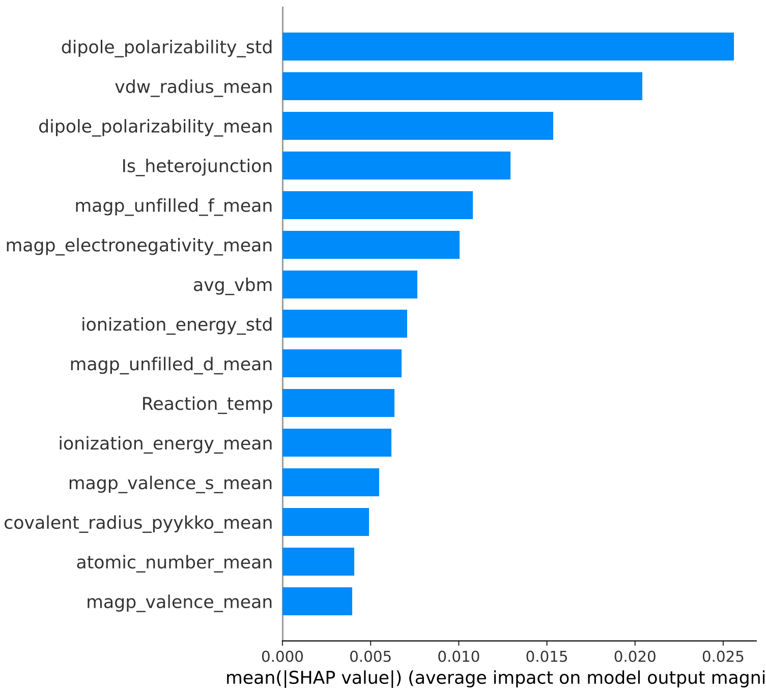
Minor Product -- Class: HCOOH
