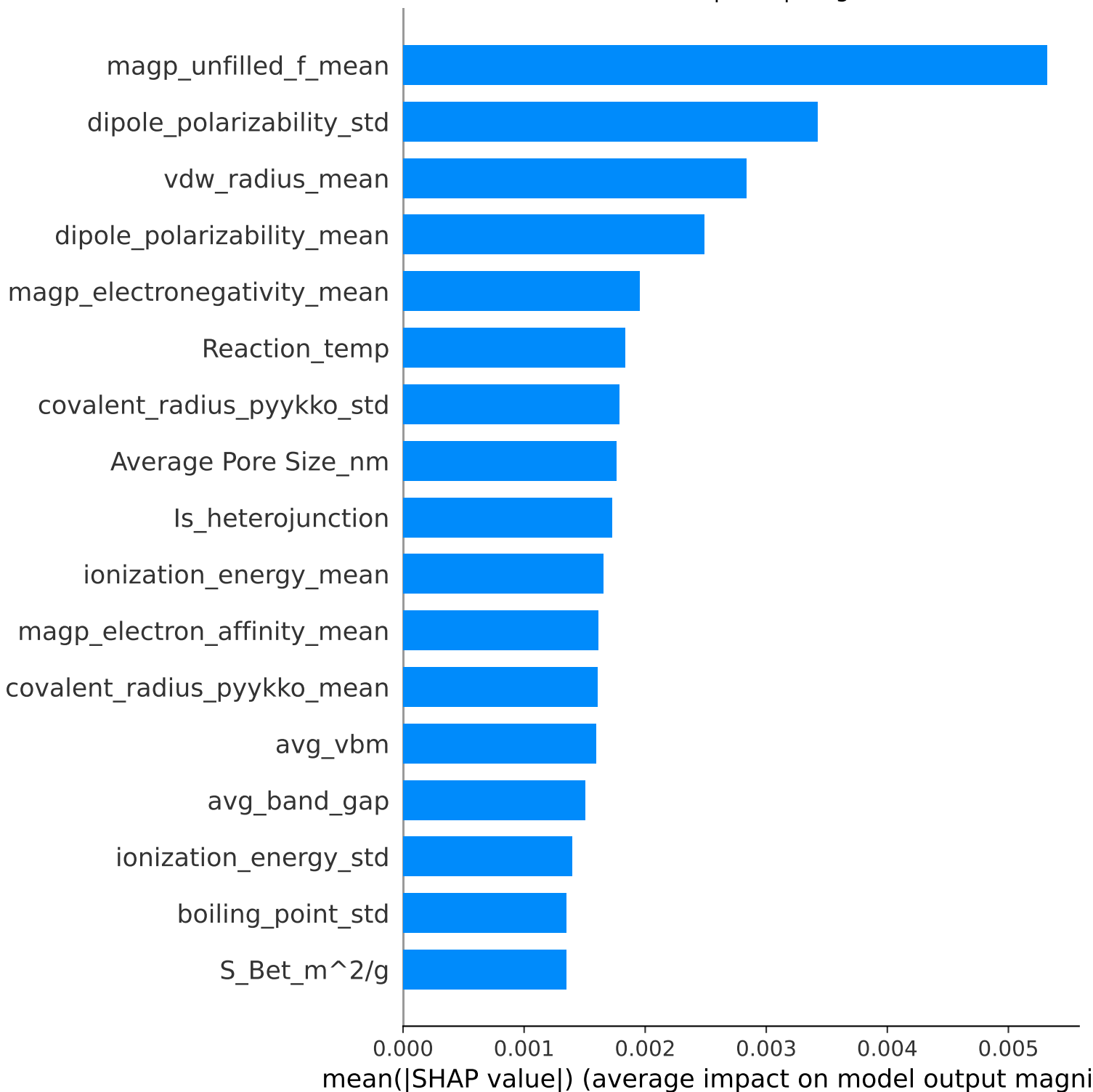
Minor Product -- Mean |SHAP| (avg across classes)
