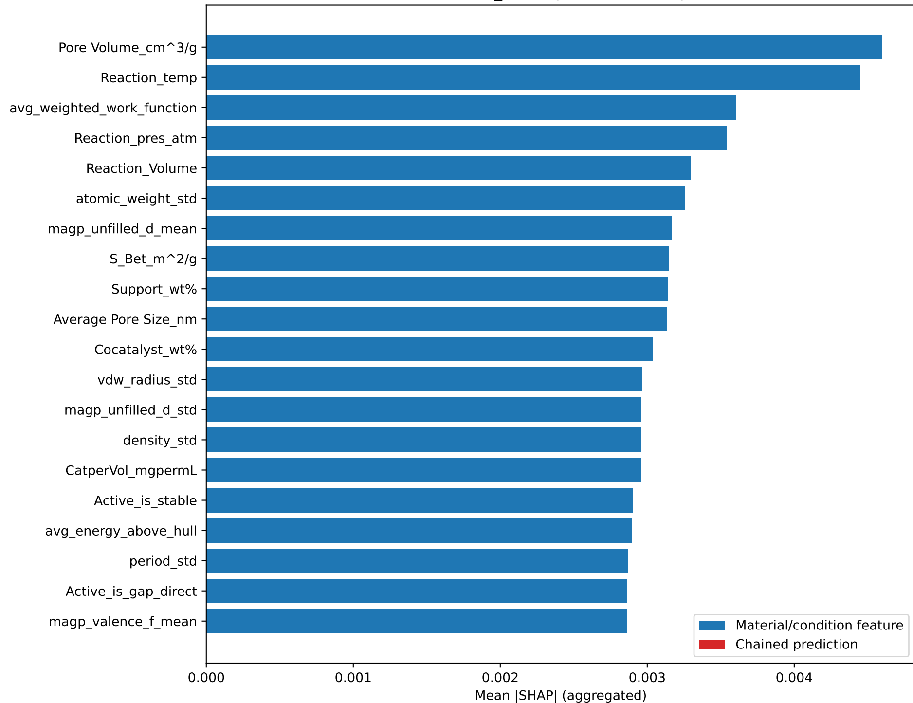
PRIDMO RF - mi_clf: Original Feature Importance
