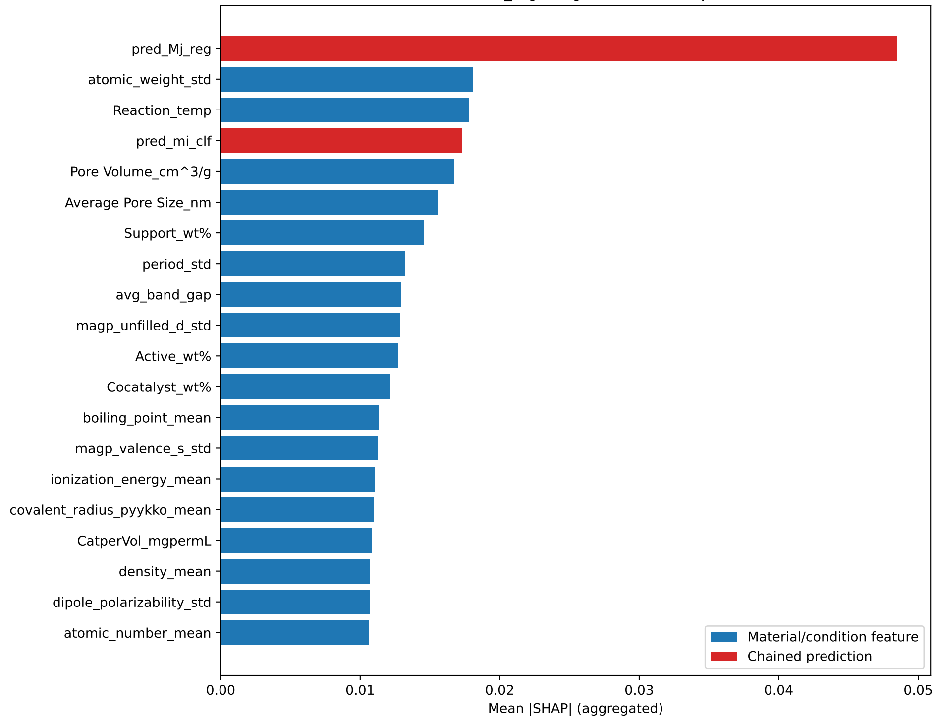
PRIDMO RF - mi_reg: Original Feature Importance
