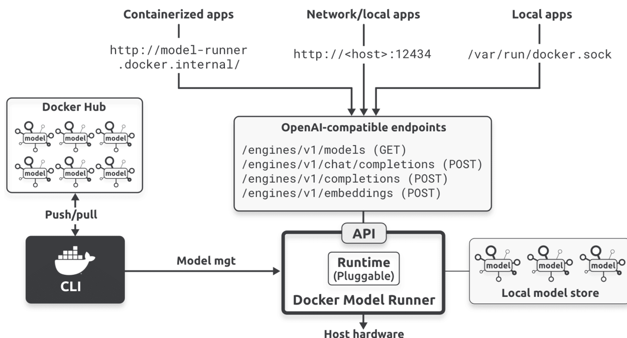
Figure 10.1 - Docker Model Runner Architecture
