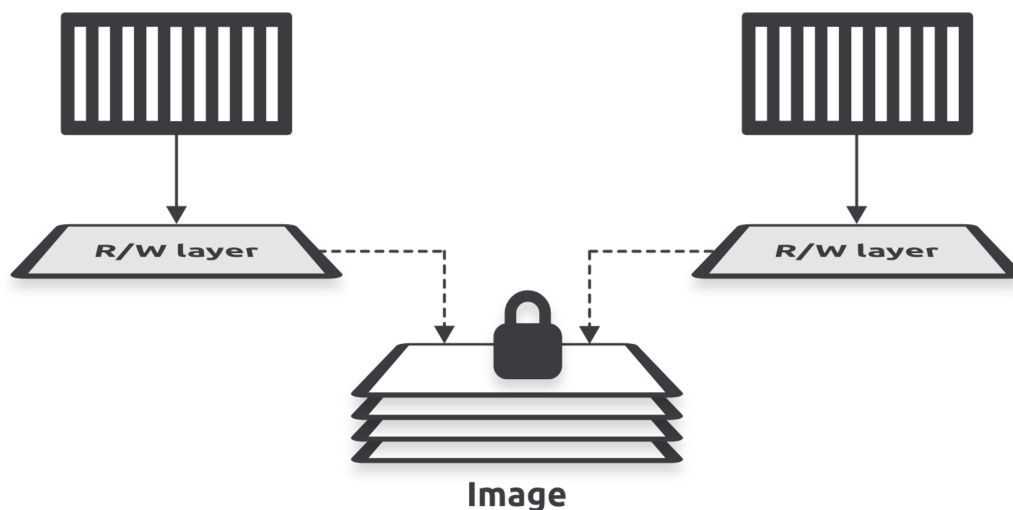
Figure 7.3 - Container R/W layers
