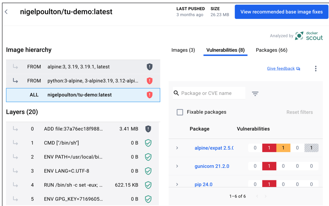
Figure 16.8 - Docker Scout integration with Docker Desktop
