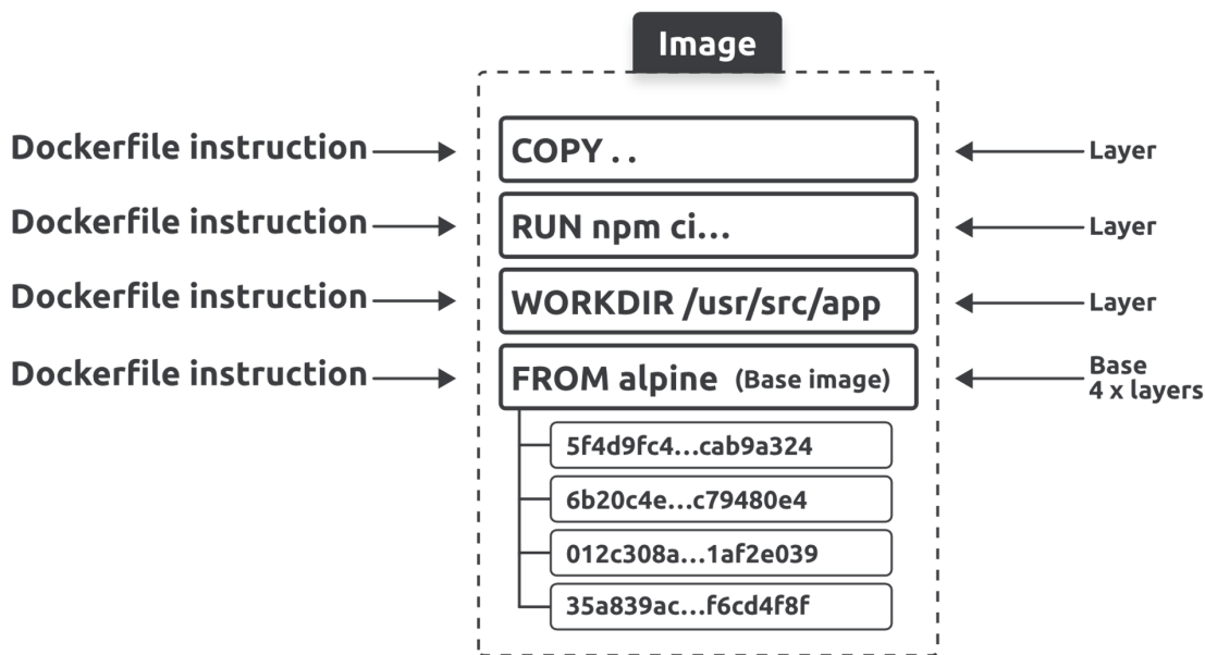
Figure 8.2 - Dockerfile and image layers
