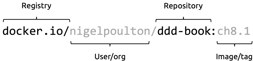
Figure 6.5 - Fully qualified image name
