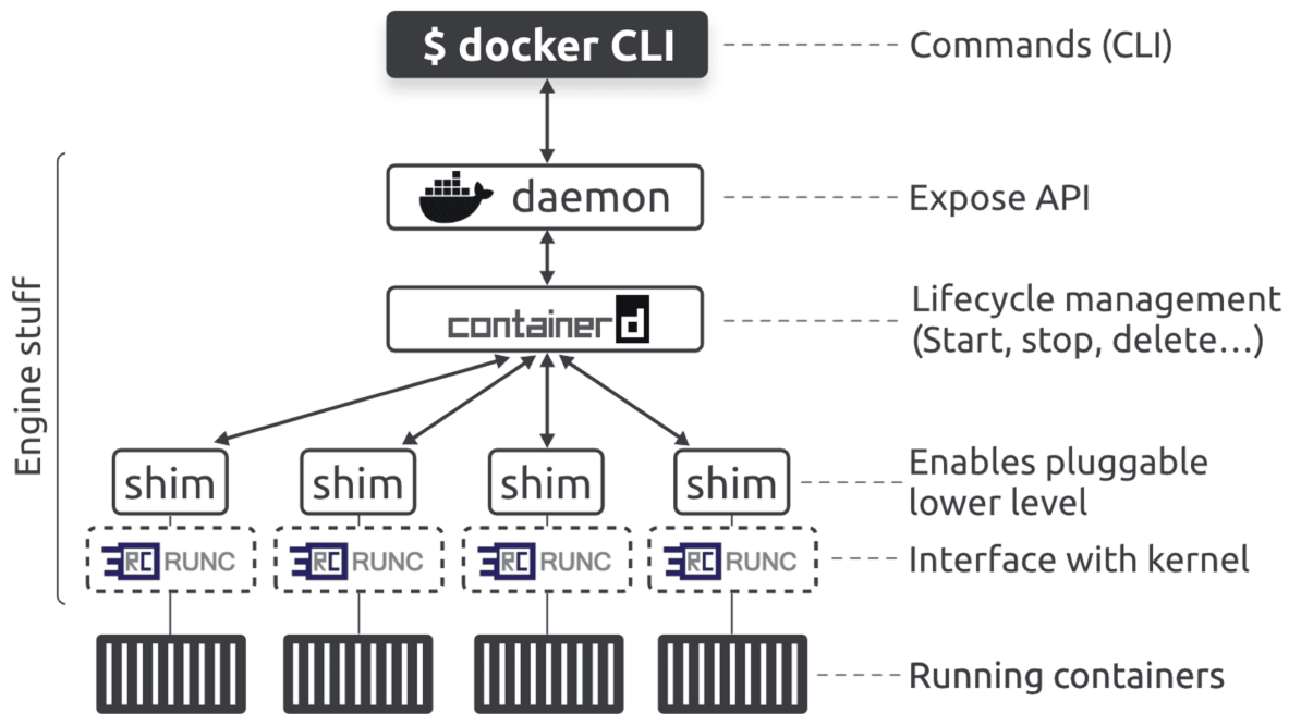
Figure 5.2 - Engine components and responsibilities
