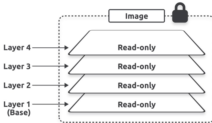
Figure 6.6 - Image and stacked layers
