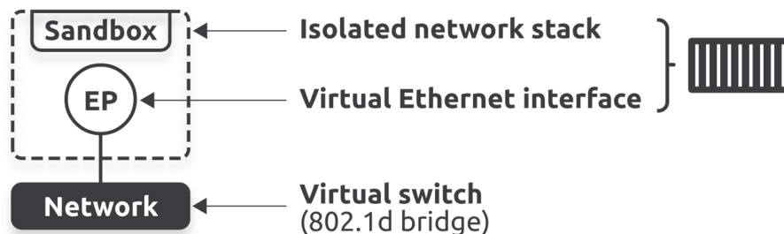
Figure 13.2 - The Container Network Model (CNM)
