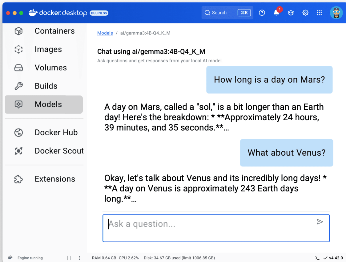
Figure 10.3 - Docker Desktop's Model Chat Window
