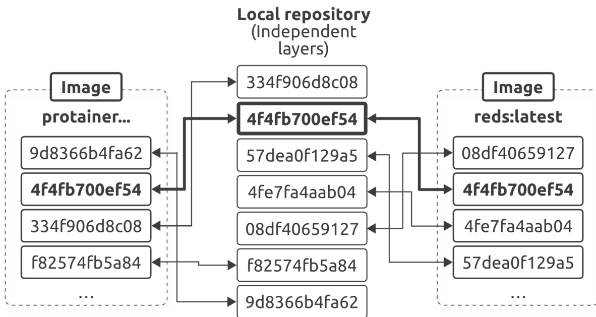
Figure 6.12 - Two images sharing a layer
