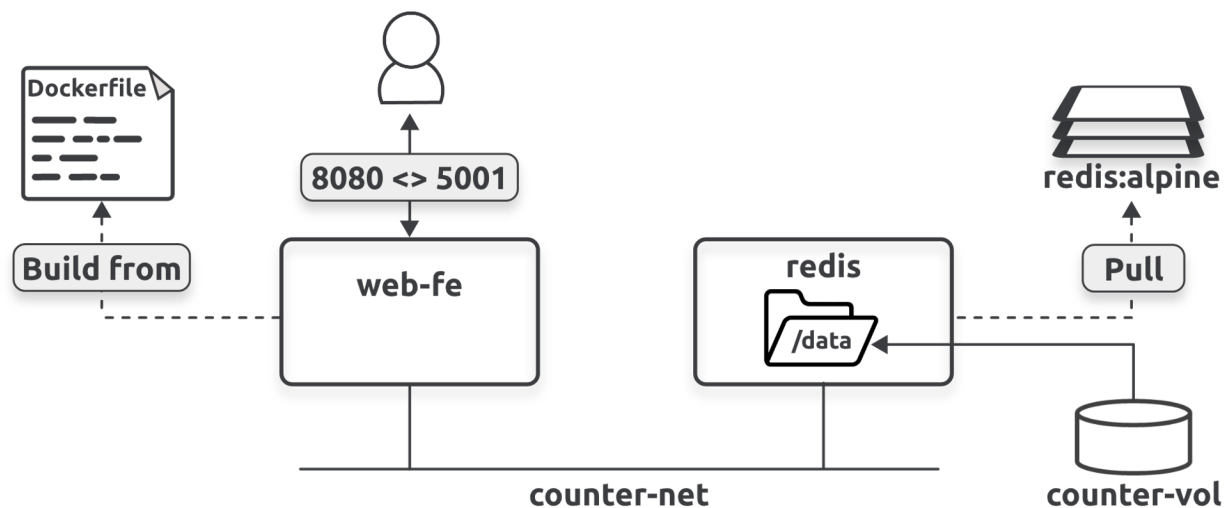
Figure 9.2 - Detailed view of sample app
