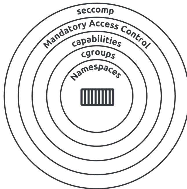
Figure 16.3 - Linux security defense in depth
