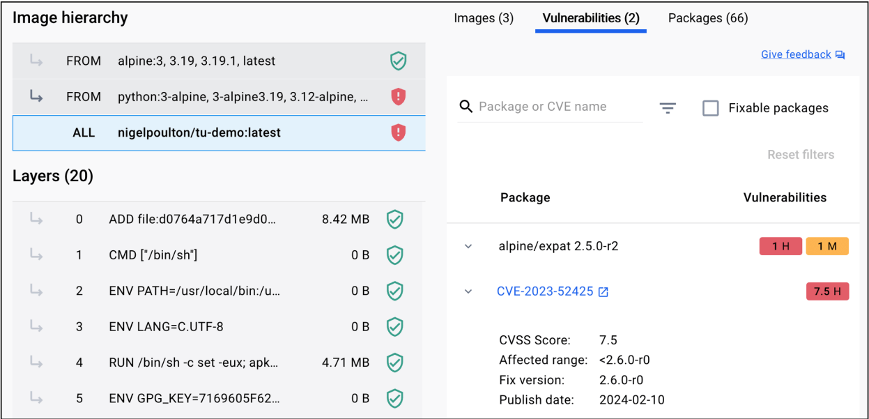
Figure 6.14 - Docker Scout integration with Docker Desktop
