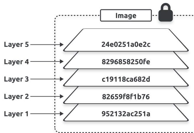
Figure 6.7 - Image layers and IDs
