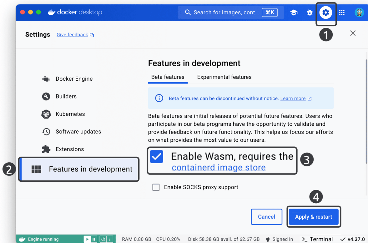
Figure 11.2 - Docker Desktop Wasm settings
