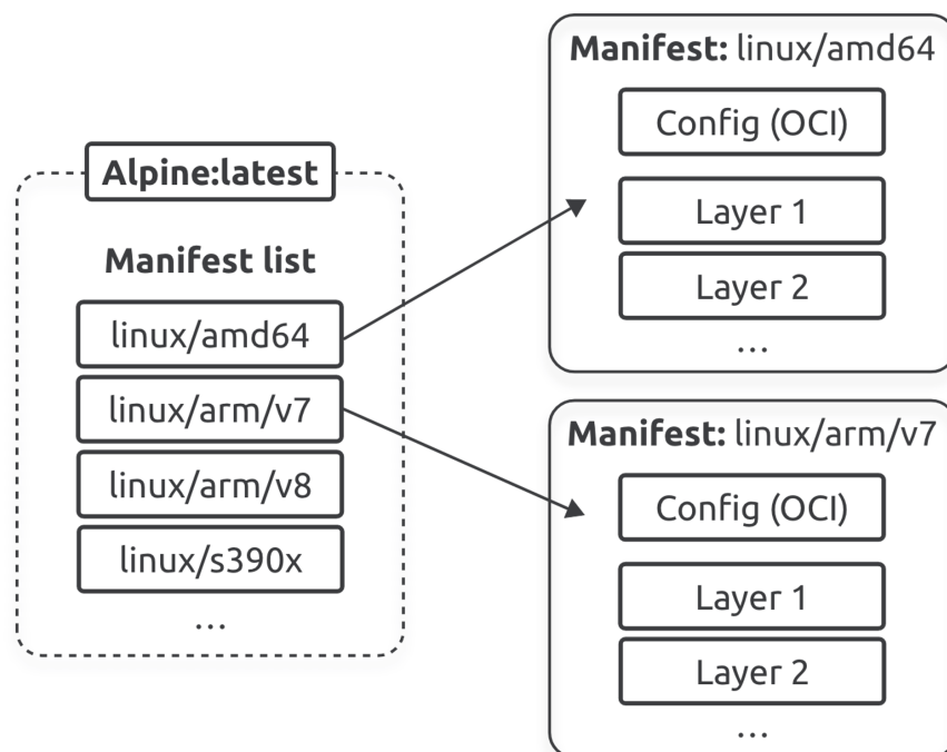
Figure 6.13 - Manifest lists and manifests
