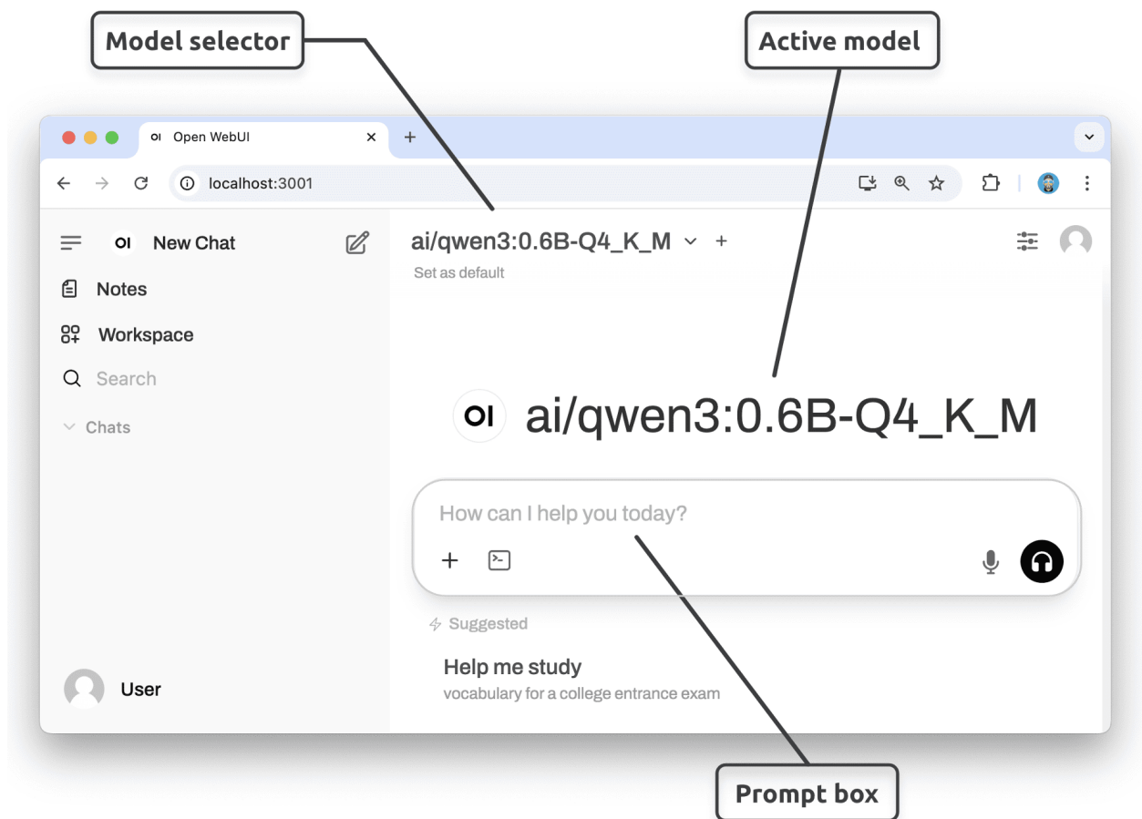
Figure 10.6 - Open WebUI interface
