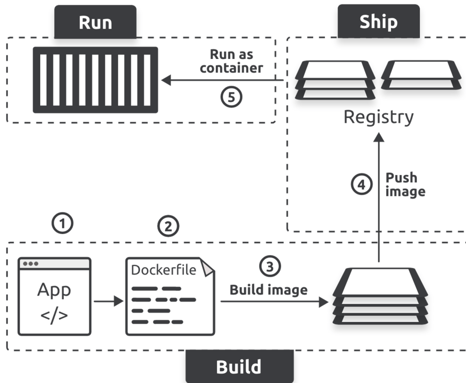
Figure 8.1 - Basic flow of containerizing an app
