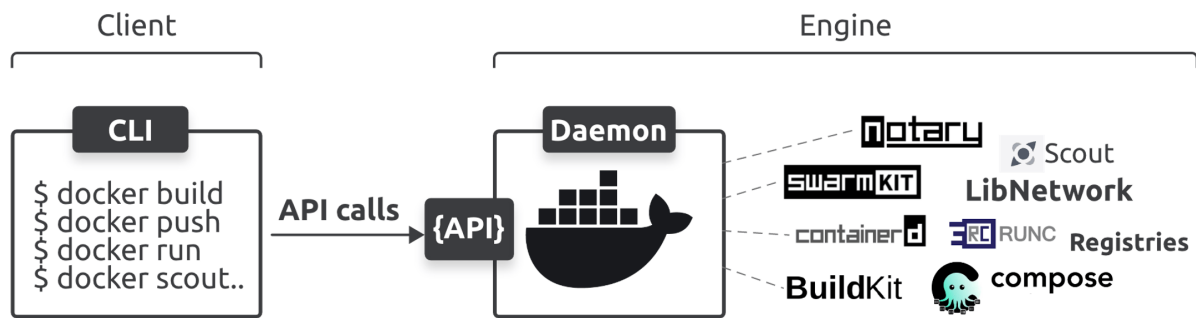
Figure 2.2 - Docker CLI and daemon hiding complexity.
