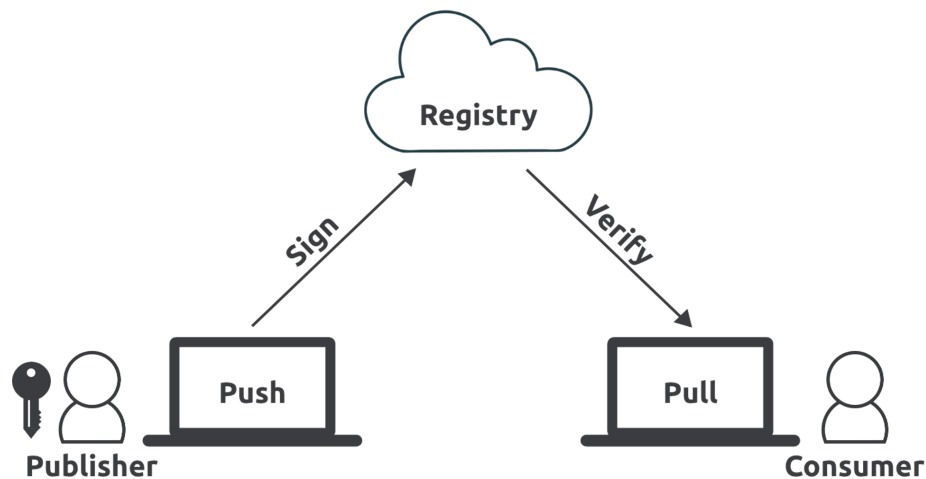
Figure 16.9 - Docker Content Trust image signing and verification
