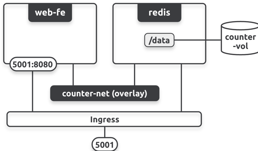
Figure 12.2 - The sample app
