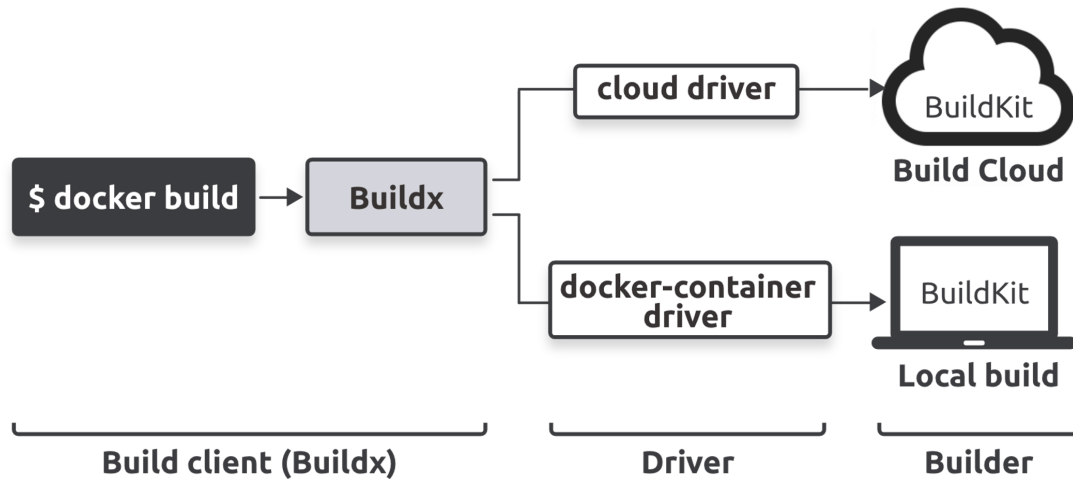
Figure 8.7 - Docker build architecture
