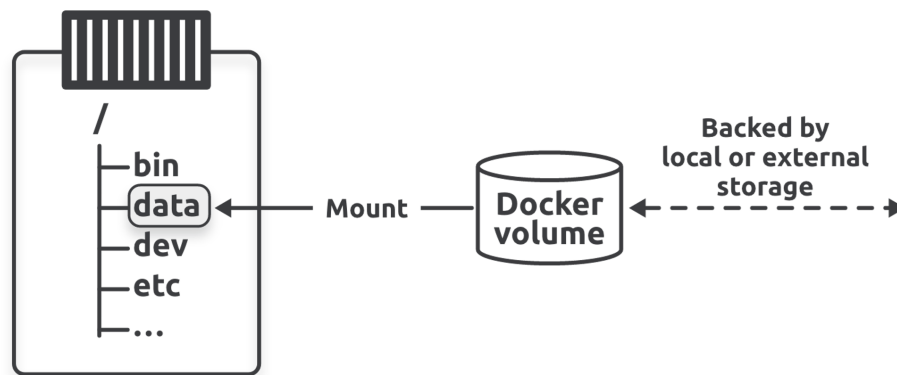
Figure 15.2 - High-level view of volumes and containers
