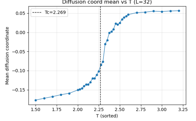
FIG. 1. The first diffusion coordinate increases monotonically with T . Notice that the region of the highest slope diagrammatically corresponds to the presence of the critical temperature.
