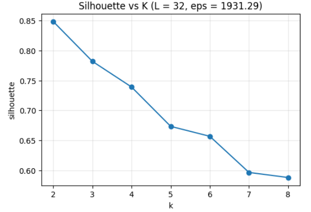
FIG. 5. XY Model Silhouette Score vs K Cluster Number ( L = 32 ).
