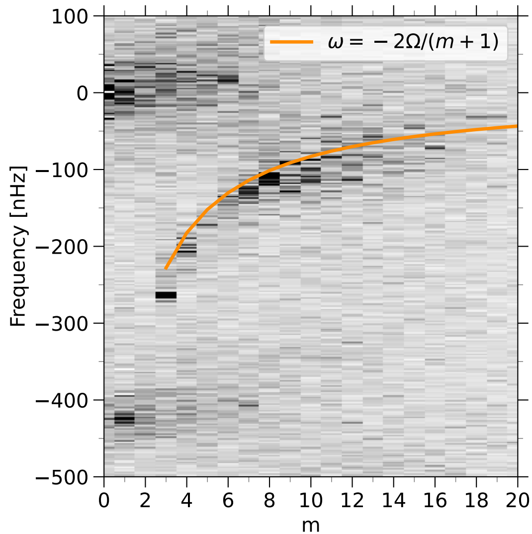
Power spectrum of u_\theta^+ (LCTMag)
