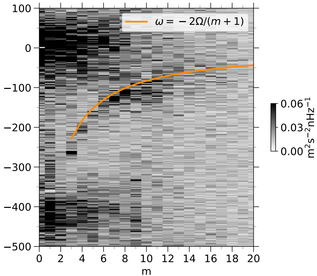
Power spectrum of u_\theta^+ (LCTGran)
