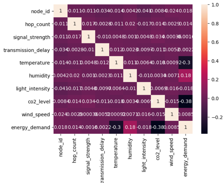
Fig 6.3: Correlation Heatmap
