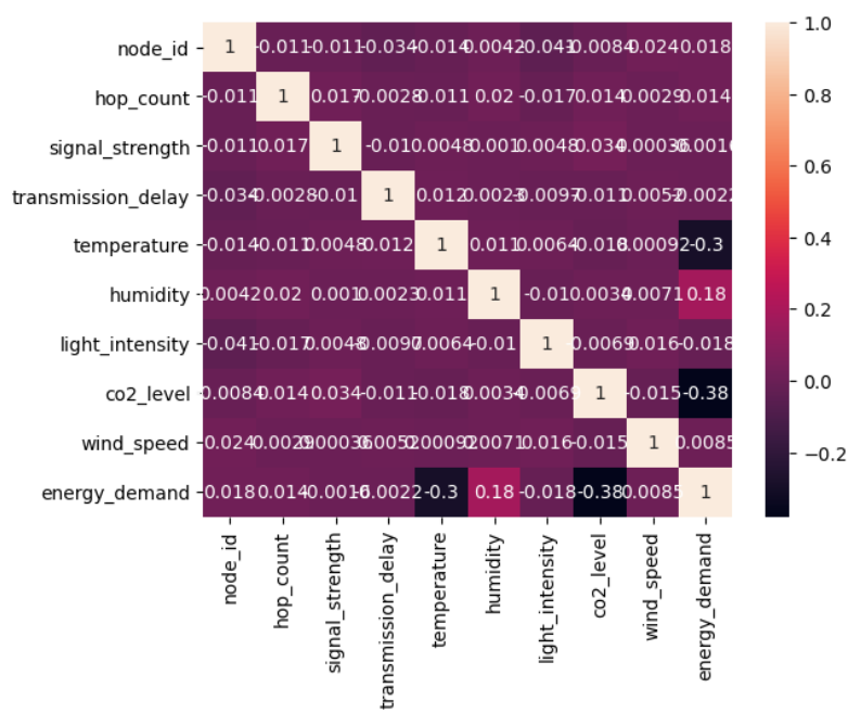
Fig 6.3: Correlation Heatmap
