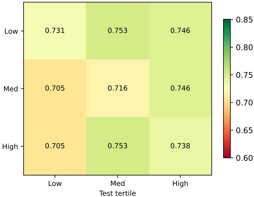
GP (c=24)
