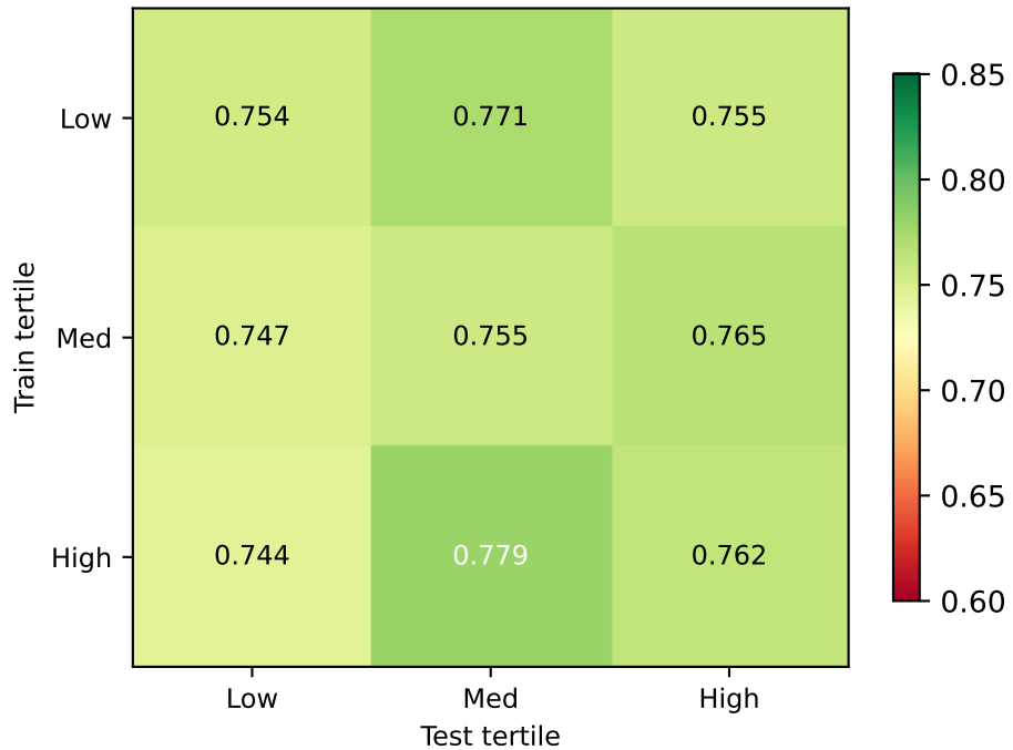
RF
