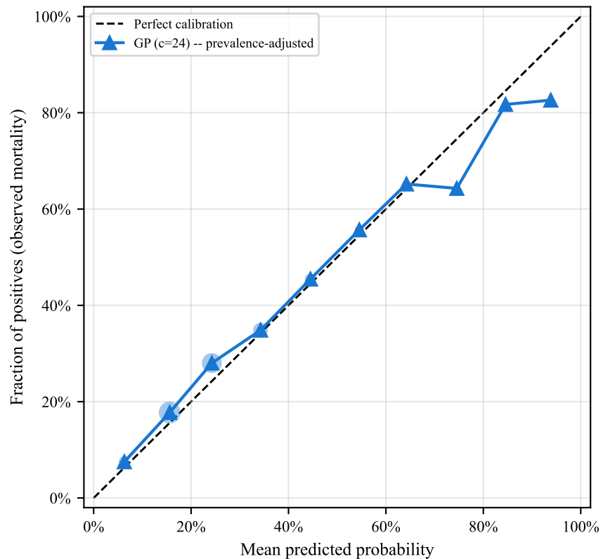
(b) Prevalence-adjusted (ECE=0.023)
