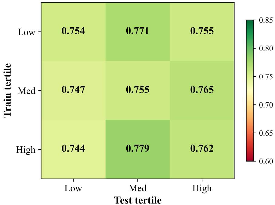
RF
