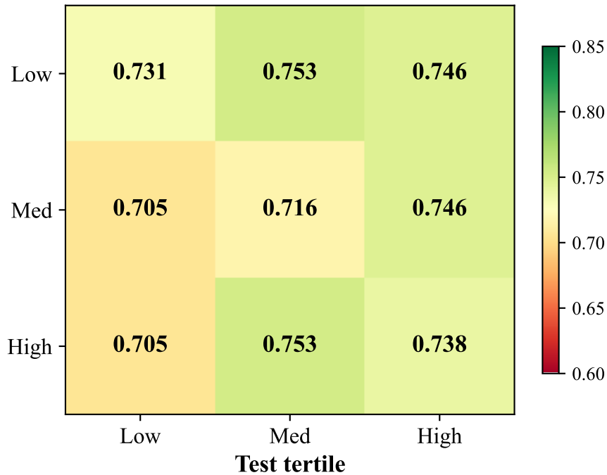
GP (c=24)
