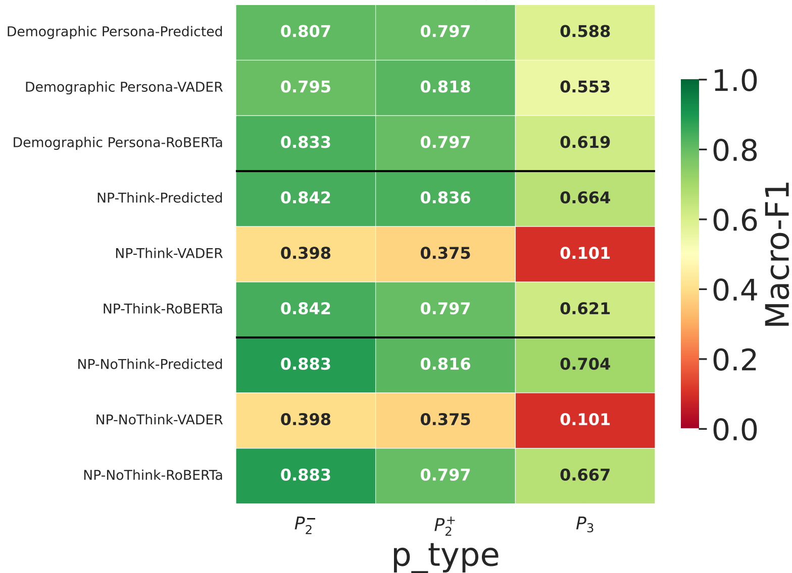
Macro-F1 vs. human ground truth ( \sigma=3 ) All conditions & approaches
