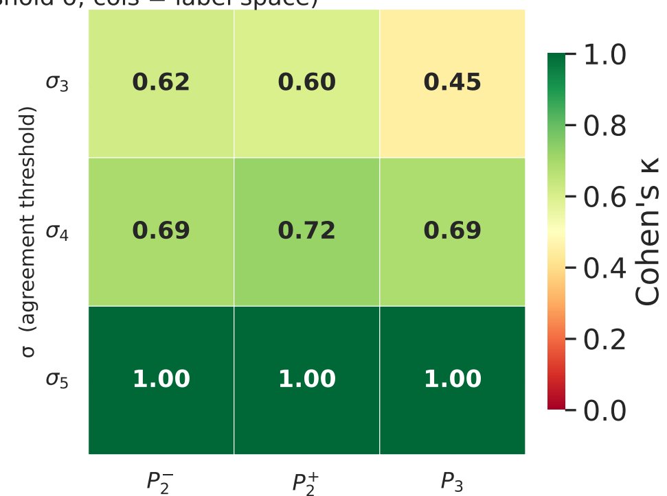
Sentiment approaches vs. PerceptSent human ground truth Predicted — Macro F1 (rows = agreement threshold \sigma ; cols = label space) Predicted — Cohen's \kappa
