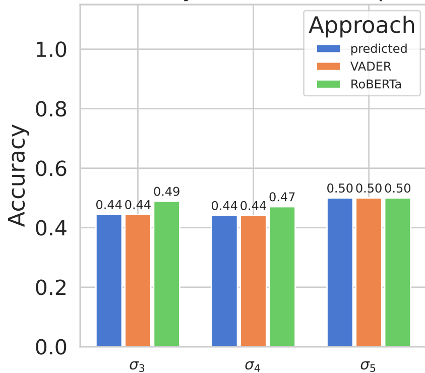
Accuracy vs. Human GT (p3)
