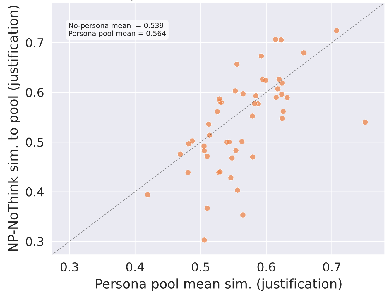
Justification — NP-NoThink
