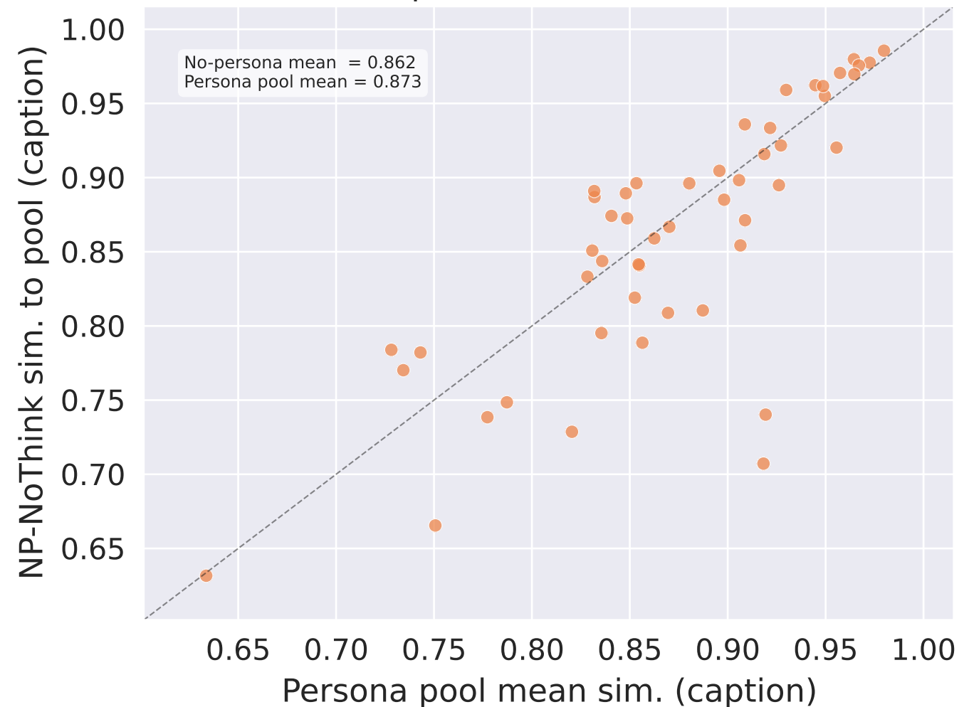
Justification — NP-NoThink
