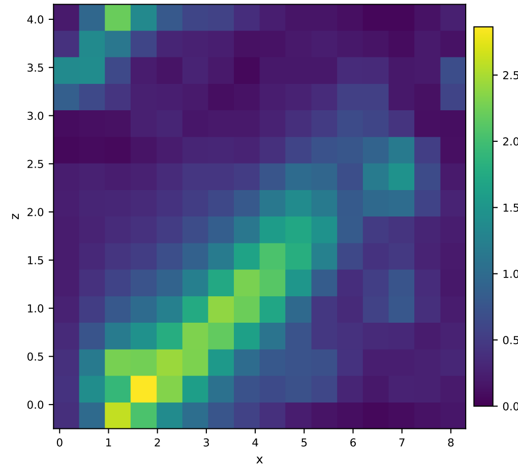
Predicted |u| at y=-0.797
