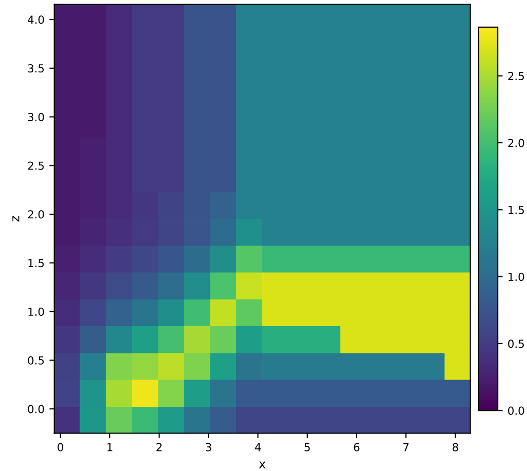
True |u| at y=-0.797
