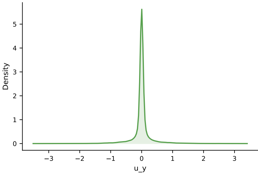
Distribution of u_y (test set)
