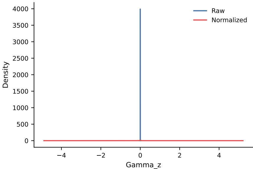
Distribution of Gamma_z
