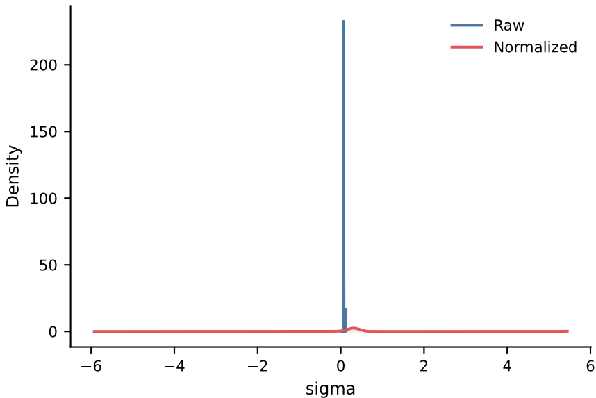
Distribution of sigma
