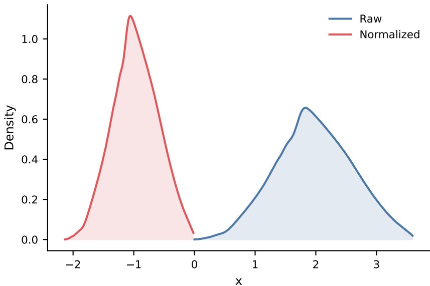
Distribution of x
