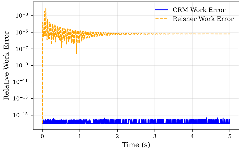
Energy Conservation Error
