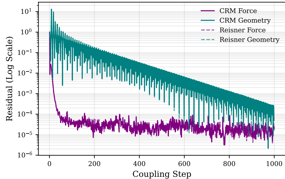
FSI Convergence
