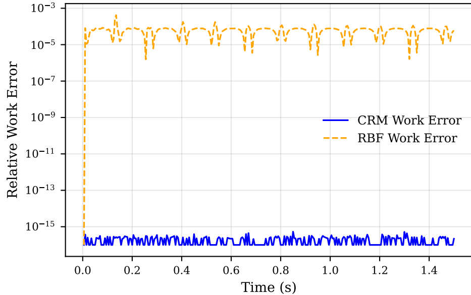
Energy Conservation Error
