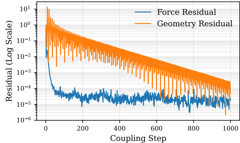
FSI Convergence
