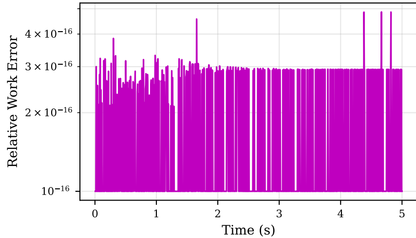
Energy Conservation Error
