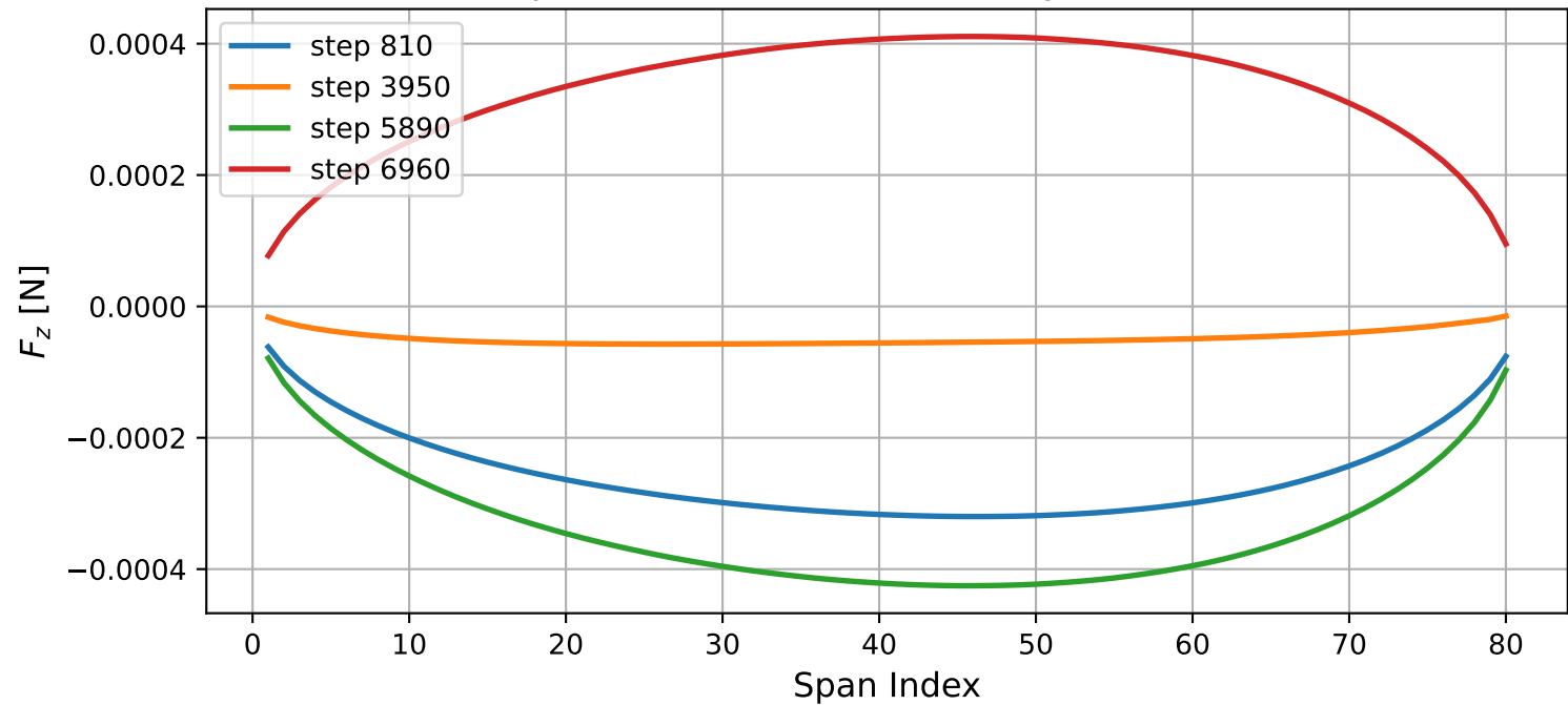
Spanwise Distribution of Payload Force
