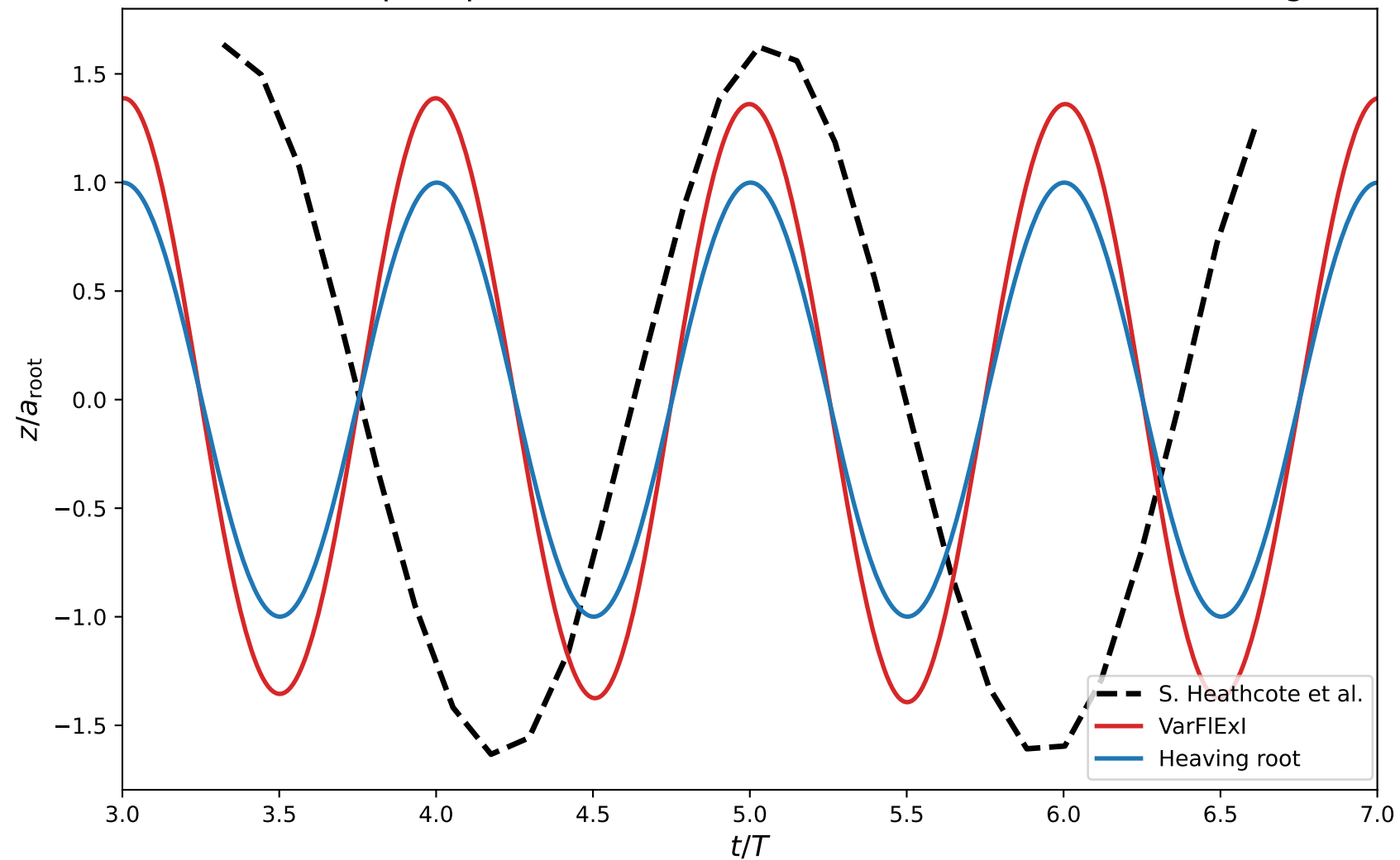
Validation of Tip Displacement: Re=30000 , U_{inf}=0.30 m/s, \rho=998\text{kg/m}^3
