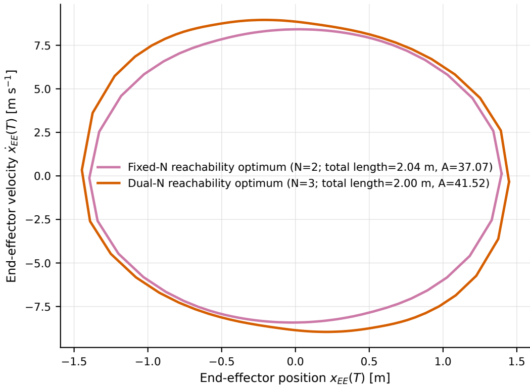
Reachability optimization comparison, T = 2 s
