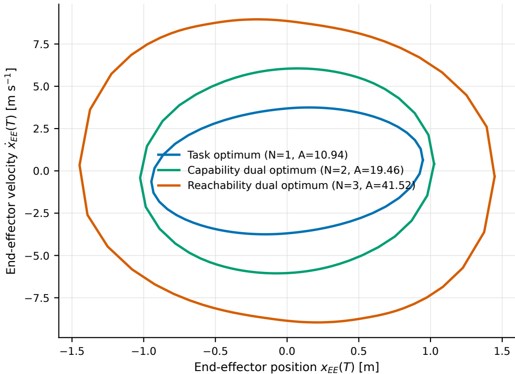
Bounded-torque reachable set at T = 2 s
