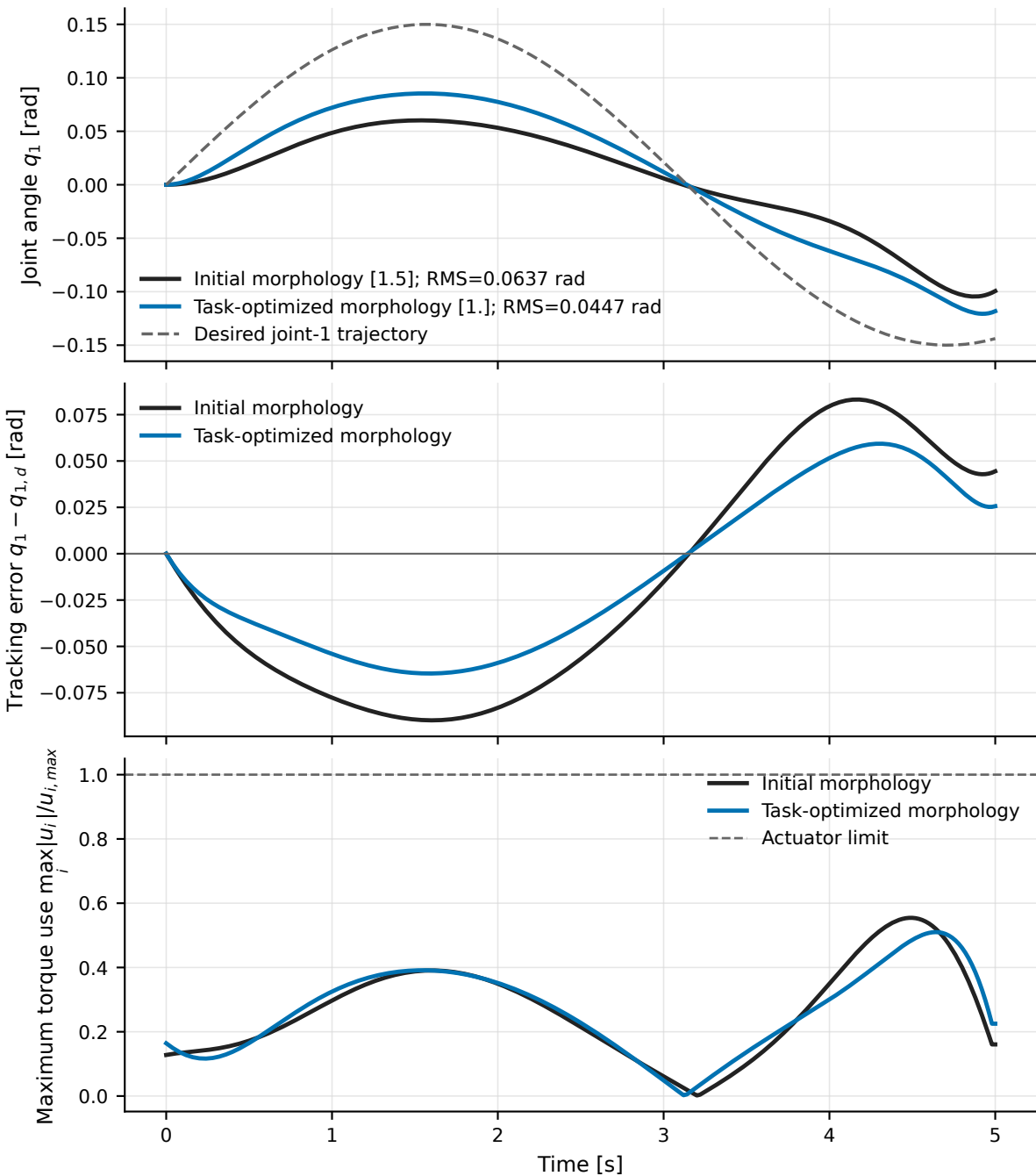
Torque-limited LQT tracking, same N=1 and torque limits
