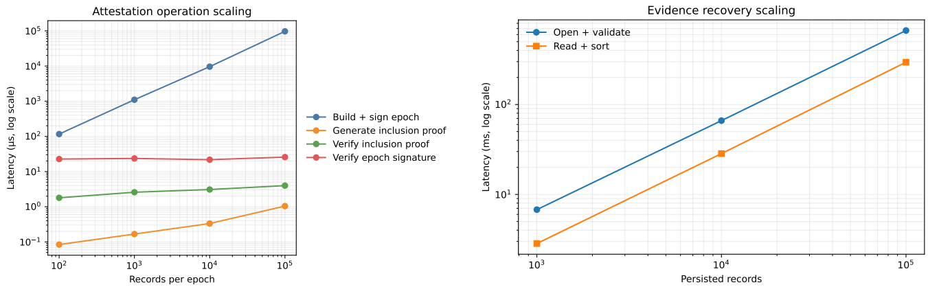
Figure 4: Canonical epoch-operation and recovery scaling. Every plotted value is derived from manifest-verified raw CSV files.
