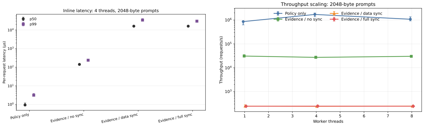
Figure 3: Inline latency and throughput from canonical raw observations. Log axes expose the orders-of-magnitude separation between policy evaluation, buffered evidence, and per-record synchronization.
