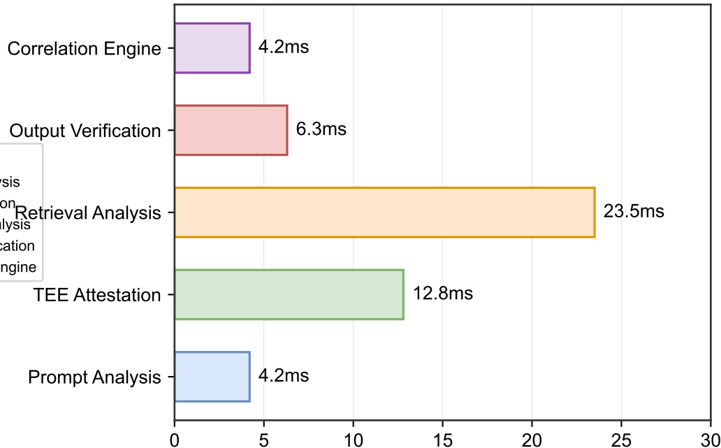
Per-Layer Latency
