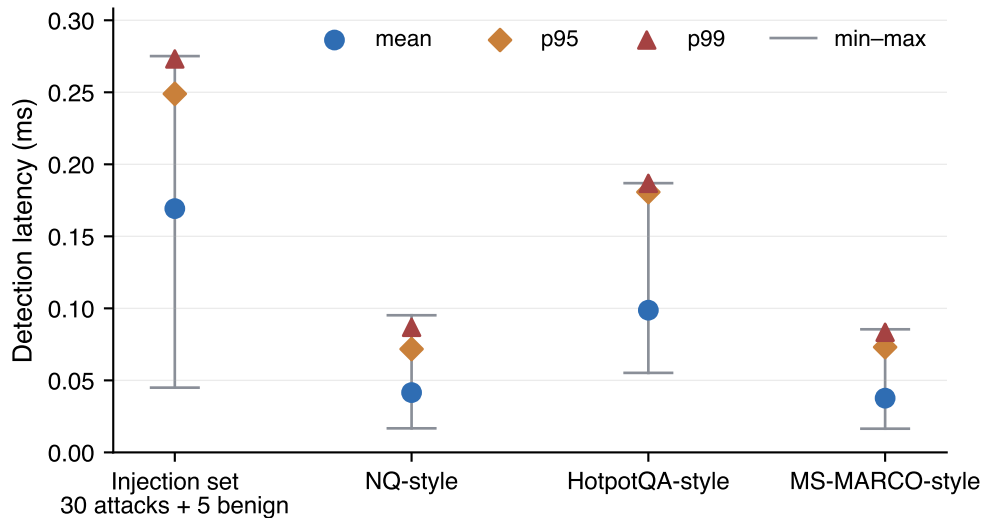
Tier-2 prompt-layer latency — 2026-07-10 (N=135, single run)
