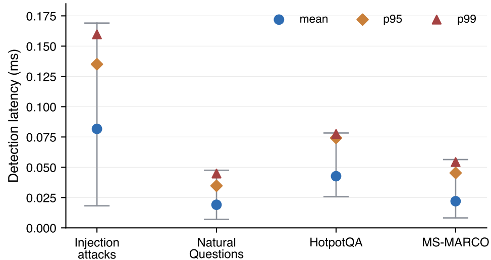
Prompt-layer detection latency by dataset (N=135, single run)
