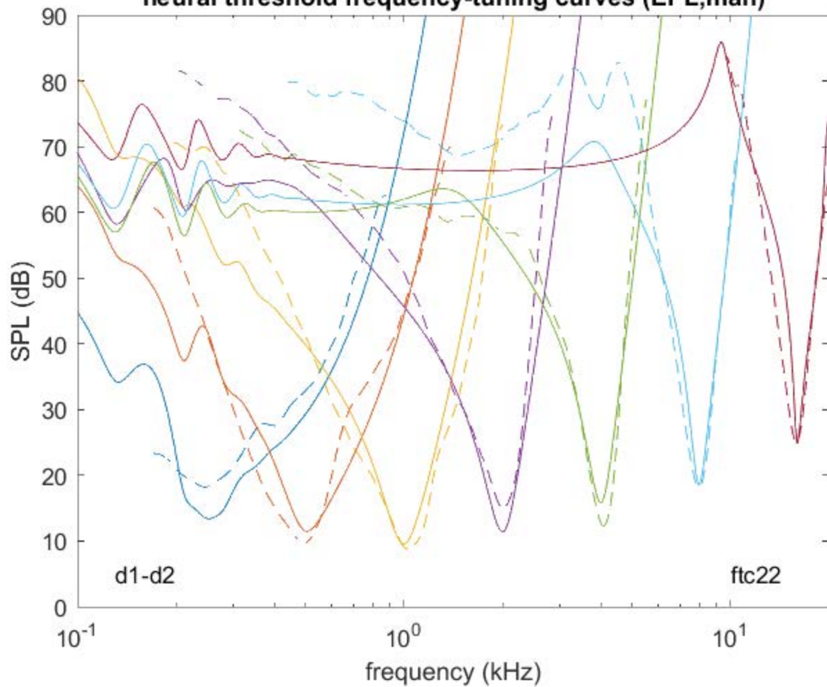
neural threshold frequency-tuning curves (EPL,man)
